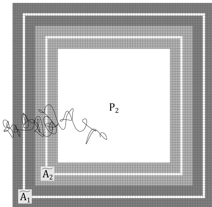
FIGURE 4.2. A decomposition P = \tilde{A}_1 \cup \dots \cup \tilde{A}_h \cup P_{hm^{d-1}} when n = 2 , m = 9 , h = 2 , and d = 1 , where each little square represents a d + 1 descendent of P . Brownian motion, started outside of P , cannot reach the inner region P_{hm^{d-1}} without passing through surfaces G_i (not displayed) drawn in the collars of white squares. Increasing h raises the number of annuli \tilde{A}_j of children of P . Increasing d yields a higher density m^{d-1} of separating surfaces per annulus.
