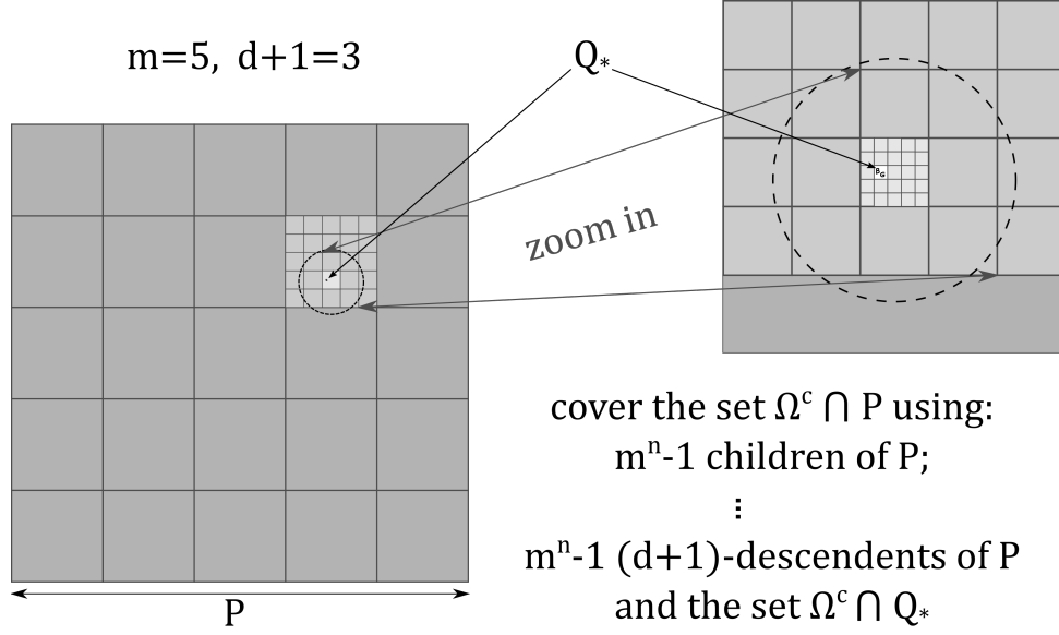
FIGURE 4.1. Optimal covering of \Omega^c \cap P under the assumption that the net content of \Omega^c inside of some (d+1) -descendent Q_* is small.
