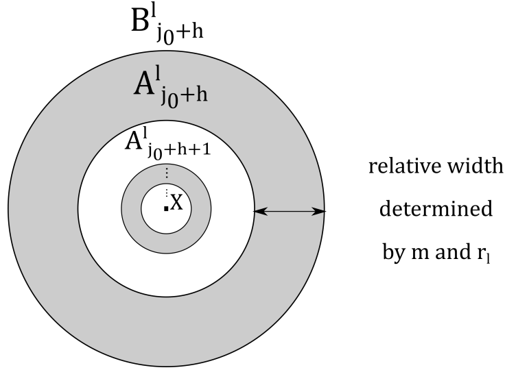
FIGURE 3.2. Annular decomposition used in the proof of (E1).
