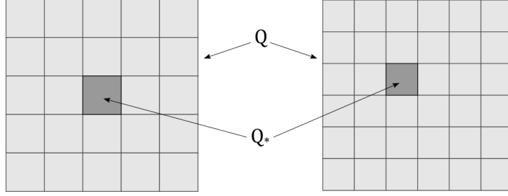
FIGURE 3.1. Examples of Q_* and Q in Lemma 3.1 when m = 5 (left) and m = 6 (right). The smaller cube Q_* is the closure of a cube P_* \in \Delta^m(\mathbb{R}^2) . The larger cube Q is the interior of a cube P \in \bar{\Delta}^m(\mathbb{R}^2) .
